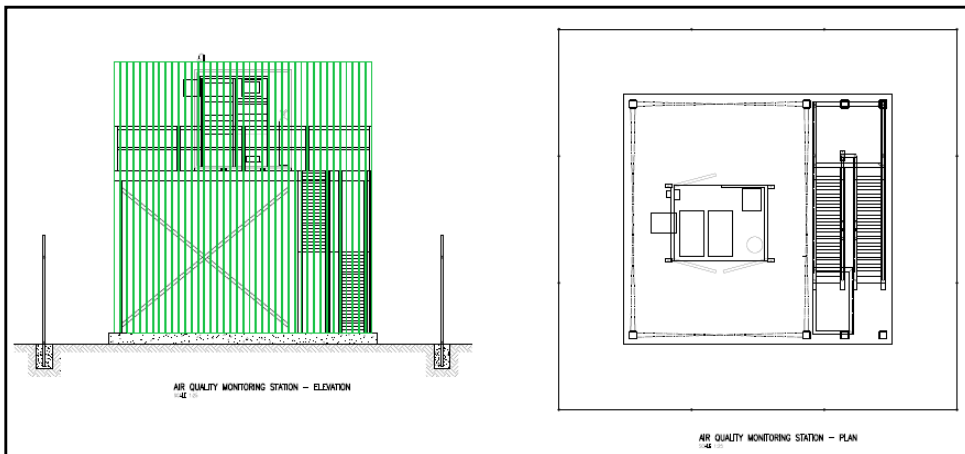
Elevation and plan view of the AQMS
